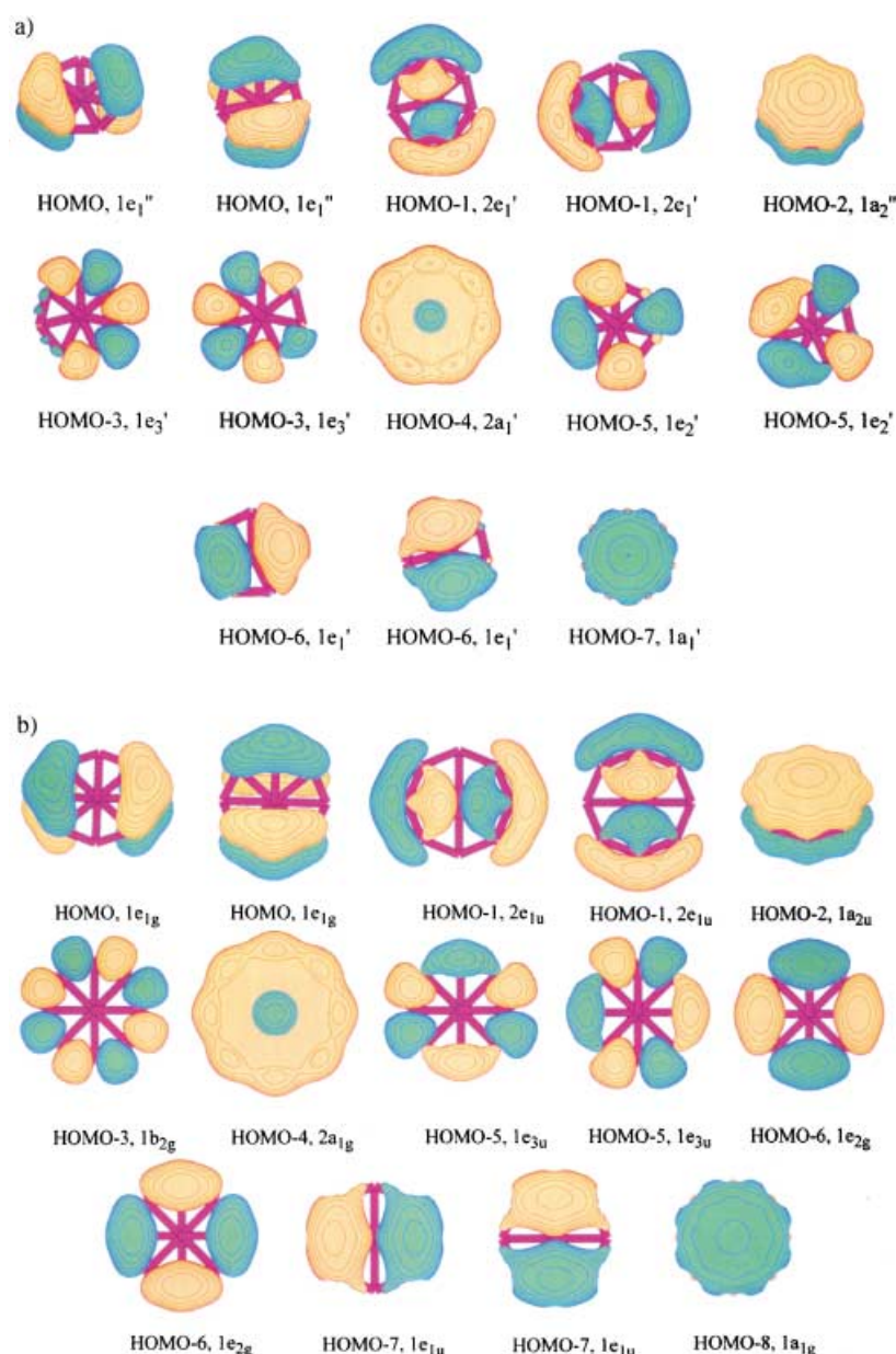
Figure 3. Molecular orbital pictures. a) D_{7h} B_8^{2-} , b) D_{8h} B_9^{2-} .
